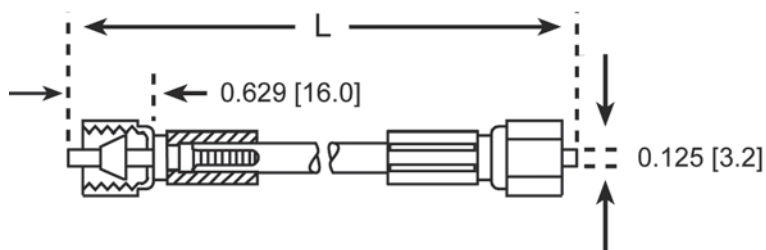
1/8 in plain adapter tip with nuts and ferrules installed
