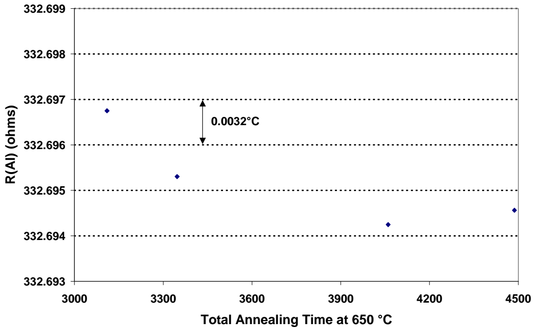
Fig. 10. The resistance R(\text{Al}) of K-2 during annealing at 650^\circ\text{C}
