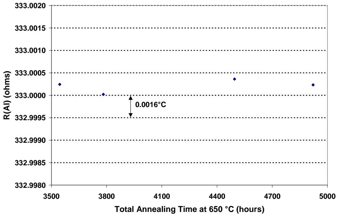
Fig. 9. The resistance R(\text{Al}) of K-1 during annealing at 650^\circ\text{C}
