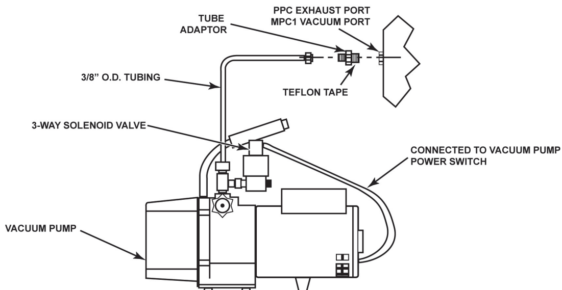
Figure 1: Fast Vac Vacuum Pump Illustrated Parts
