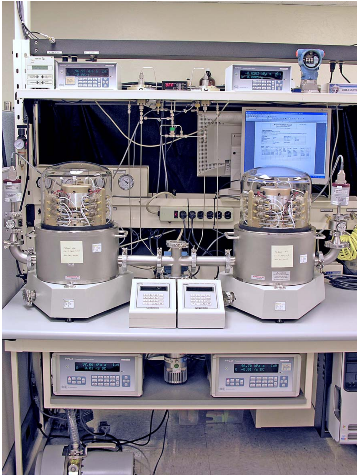
Figure 4. Picture of the automated crossfloat system at DHI
