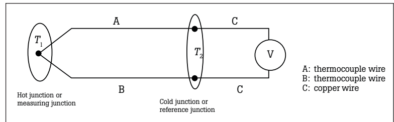
Figure 1: Thermocouple construction.
